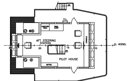
PILOTHOUSE ARRANGEMENT
