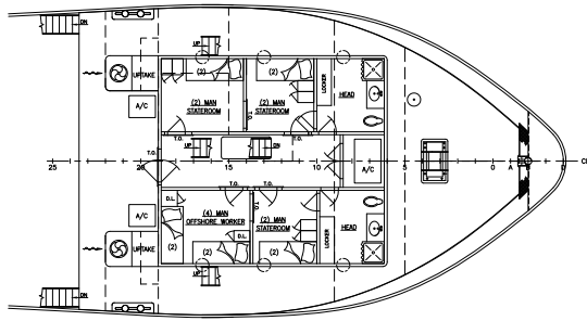
FOCSLE DECK
