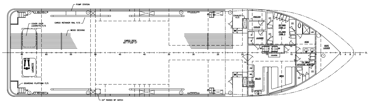
MAIN DECK
