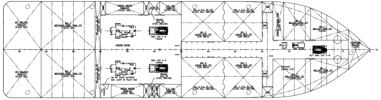
HOLD PLAN
