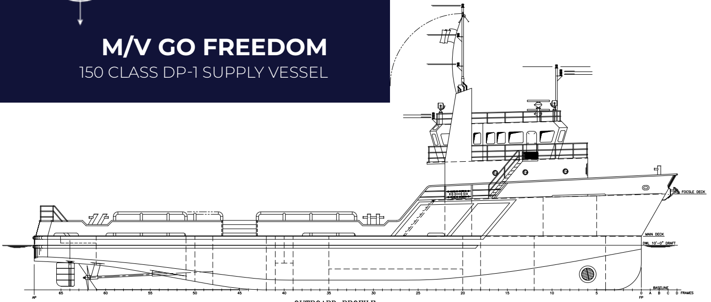
OUTBOARD PROFILE
