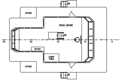
BRIDGE DECK
